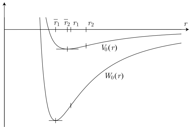
Fig. 1 Van der Waals forces: plot of V_0 and W_0 with p = 2.25 and q = 3.5 . Condition (6.2) is satisfied since r_2/2 \approx 0.923723 < \bar{r}_1 \approx 1.15726
